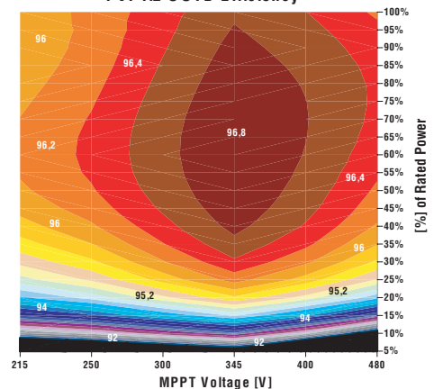
PVI-4.2-OUTD Efficiency
